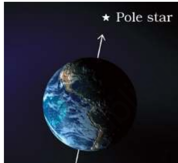
Fig 17.10: The Pole star lies close to the axis of rotation of the Earth
