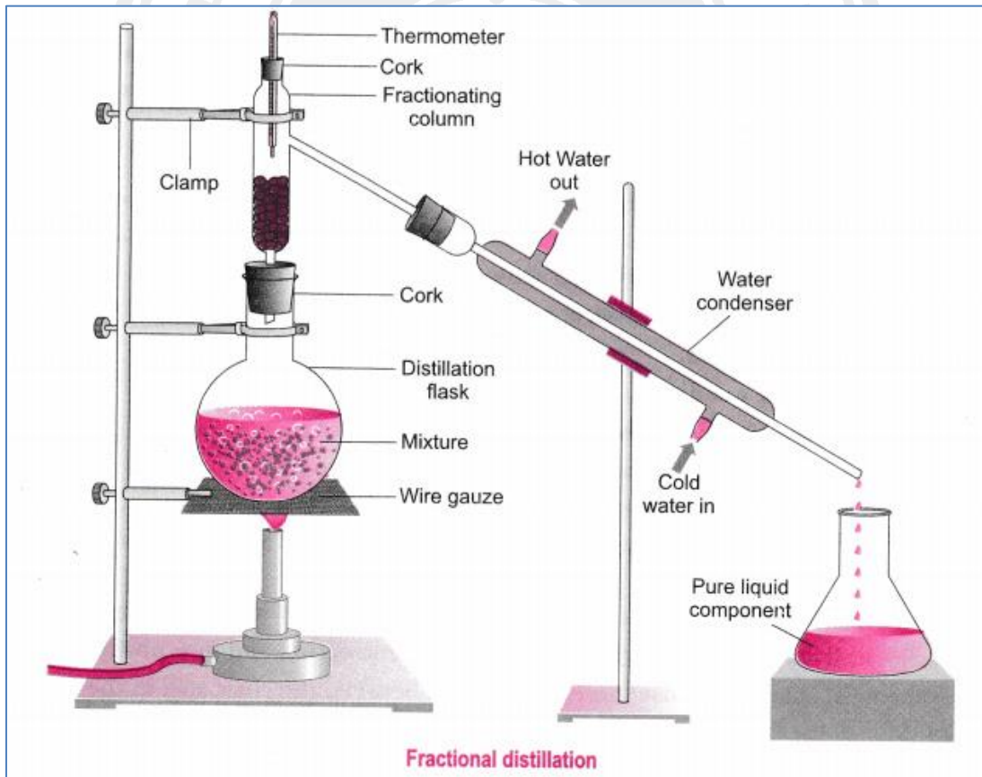
Fig. Fractional Distillation
